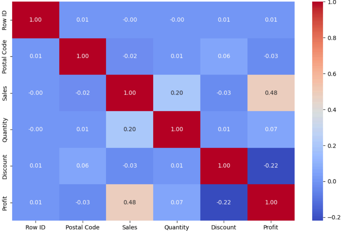
Correlation Heatmap
